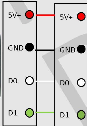
Card Reader
